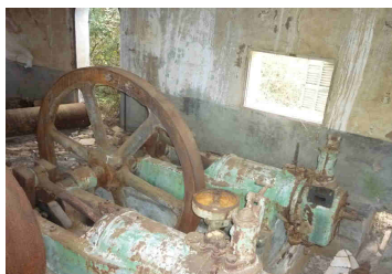
Motor "Crossley Brothers" de gas pobre
